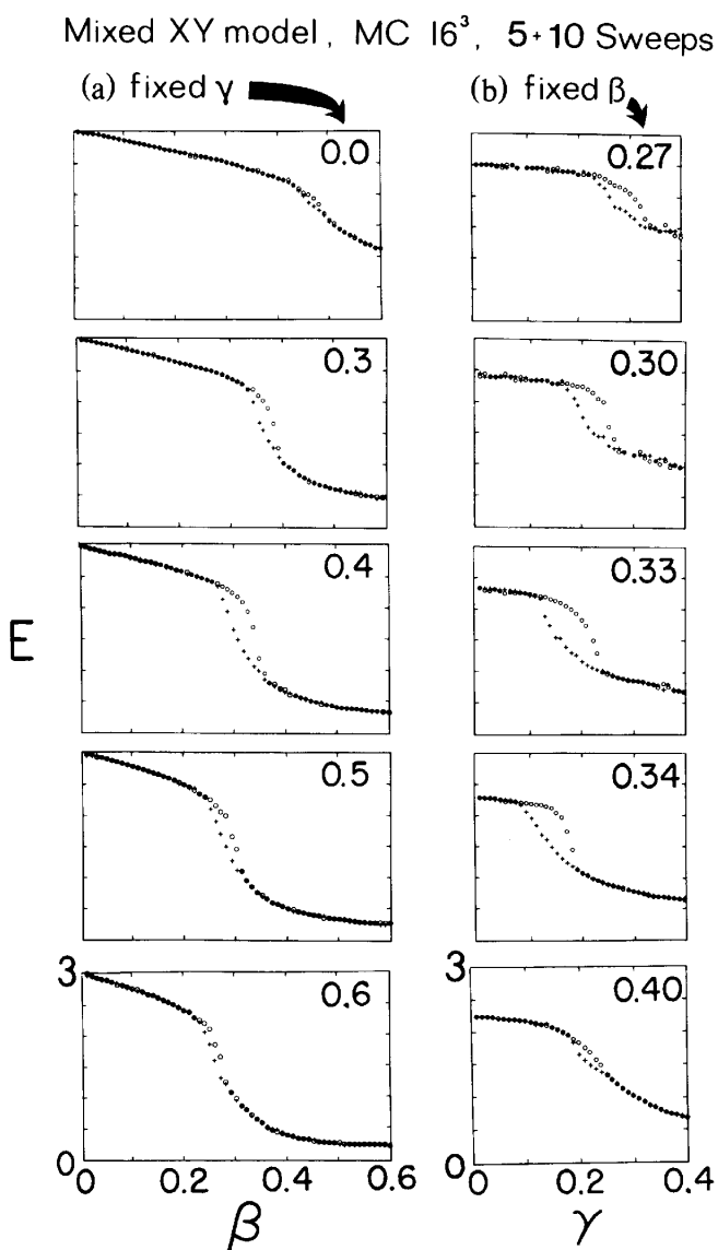
FIG. 2. (a) Thermal cycles in \beta for various fixed \gamma showing a hysteresis at \gamma \approx 0.30-0.40 as a rough indication for a first-order transition. (b) Thermal cycles in \gamma for various fixed \beta showing a hysteresis at \beta \approx 0.30-0.35 .
