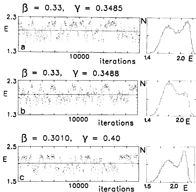
FIG. 3. The time evolution of the internal energy on a 16^3 lattice at three different points (\beta, \gamma) near the transition line. They show the jumping back and forth between two minima separated by a barrier typical for a first-order transition. At the right end of each evolution diagram we show the corresponding histograms displaying clearly the double peak of a first-order transition.
