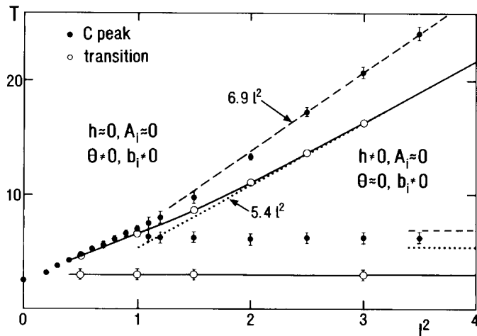
FIG. 1. The phase diagram of the lattice-defect melting model for \nu=1 . The abscissa is the square of the length scale of rotational stiffness, and the ordinate, the temperature. The transition points are determined from measurements of correlation functions on 32 \times 32 lattices. In the hot phases we have indicated the roughness of the integer field configurations h, A_i and the defects as in Ref. 7. The lower phase contains very few defects and is completely rough in h and A_i . On the right-hand margin we have indicated the position of the specific-heat peak and the Kosterlitz-Thouless transition for l=\infty . At finite l , the transition temperatures are lower by a factor of about 2 since the longitudinal mode has only a finite range l and does not contribute to the critical limit of the renormalization flow. The peak in the specific heat has only small 1/l^2 corrections.
