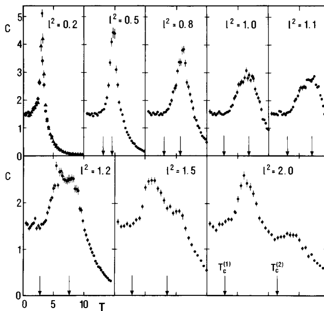
FIG. 2. The specific heat vs temperature of the defect melting model on a 16 \times 16 lattice with increasing length scale of rotational stiffness l . In all plots, the temperature scale is the same. The arrows indicate the transition points which, for l^2 > 1 , lie clearly below the peaks. It is not necessary to plot the peaks for larger l^2 since they follow quite well the appropriately rescaled specific-heat curves of the ordinary DG model. The data are averages over 5000 configurations, after discarding 1000 configurations for thermalization.
