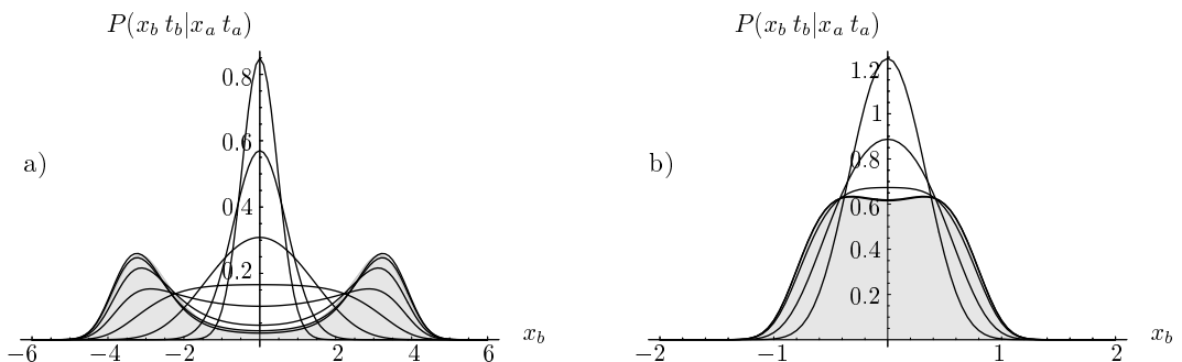
FIG. 3: Conditional probability density P(x_b t_b | x_a t_a) above the laser threshold at \kappa = -1 , D = 1 , and x_a = t_a = 0 . For the coupling constants g = 0.1 in a) and g = 10 in b) the distribution is shown for the times t_b = 0.1, 0.2, 0.5, 1, 1.5, 2, 3, 4 and t_b = 0.05, 0.1, 0.2, 0.5 from the top to the bottom at the origin, respectively.
