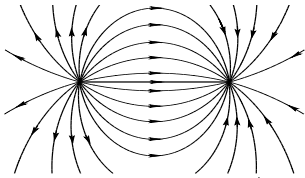
FIG. 1: Flow lines corresponding to the Dirac proposal for the external current J_\mu(z) specified by Eqs. (7) in two dimensions.
