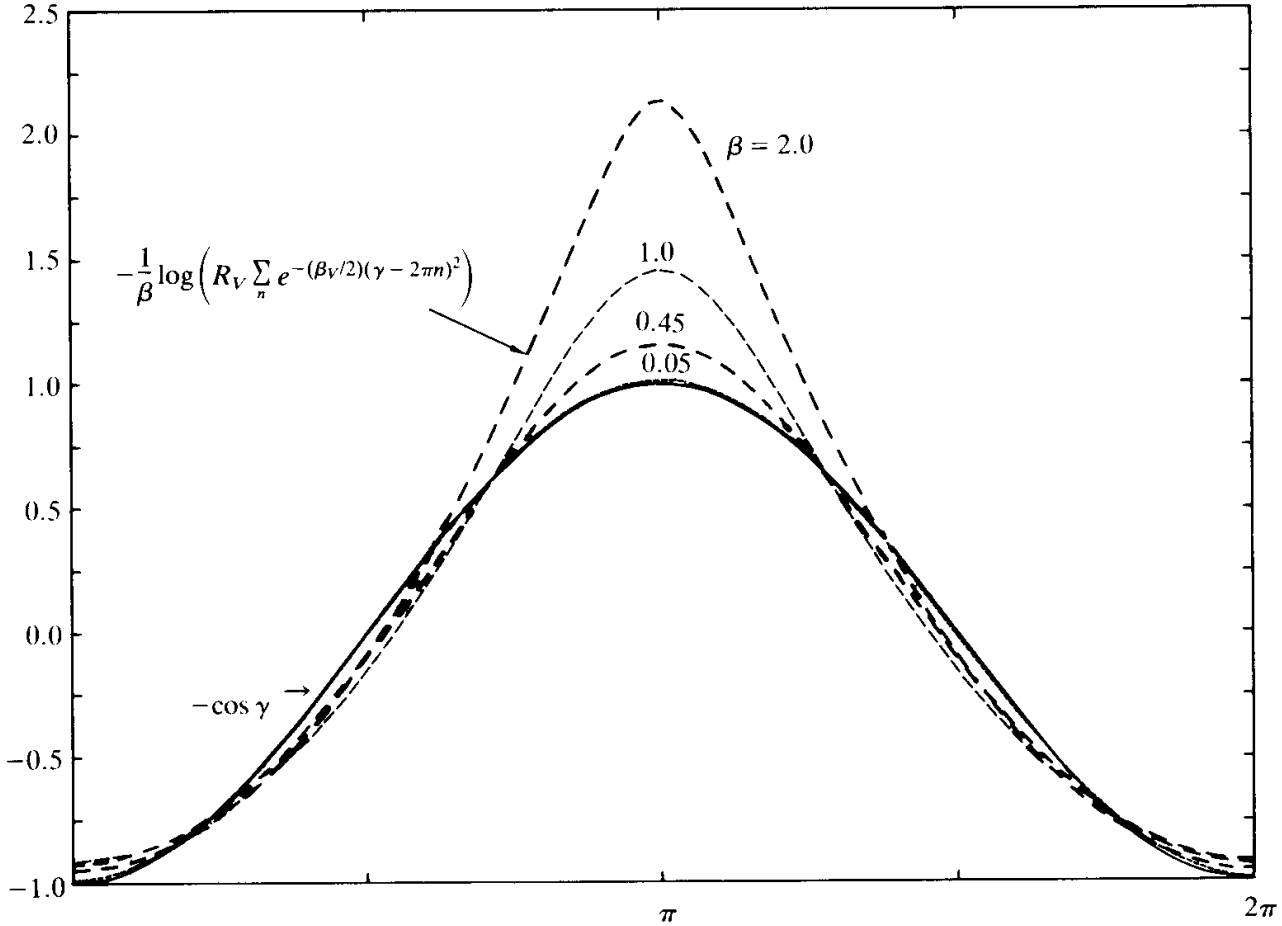
FIG. 7.4. The energy in the approximated Villain Boltzmann factors (----) as compared with the XY model (—).
