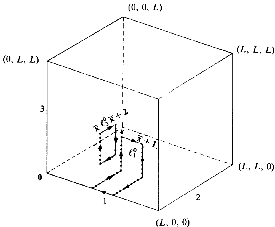
FIG. 6.3. Illustration of the construction of closed loops \bar{\nabla}_i \ell_i(\mathbf{x}) = 0 from a sum over arbitrary line pieces \ell_1^0(\mathbf{x}), \ell_2^0(\mathbf{x}) in the gauge A_3 \equiv 0, A_2(x_1, x_2, 0) = 0, A_1(x_1, 0, 0) = 0 . For details see Eqs. (6.42)–(6.47).
